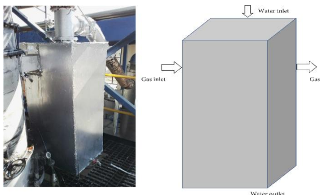
Fig.1 Heat exchanger's Pictorial and schematic view [5].
